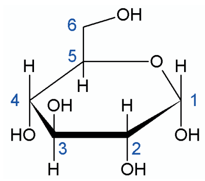
\alpha -D-glucose
